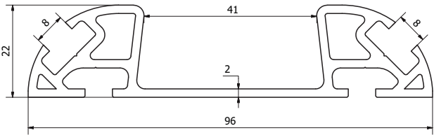
MONORAIL 40 mm
