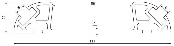
MONORAIL 55 mm
